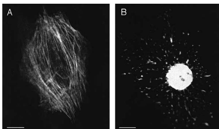
Fig. 2. Confocal images of endothelial cells stained with a microfilament-specific fluorescent probe. A: FITC-phalloidin stained control cell. Cells were fixed (see Section 2) and stained with 160 nM FITC-conjugated phalloidin (20 min) to visualize the organized F-actin microfilament network. B: FITC-phalloidin staining of cytochalasin D-treated cell. Cells were incubated with 20 \mu\text{M} cytochalasin D (to disrupt the microfilament network) for 3 h at 37°C, then fixed and stained as in (A). The image was recorded at high gain settings in order to visualize the outline of the cell and the faint remaining FITC-phalloidin fluorescence in the cell periphery after disruption of the actin filaments by cytochalasin. With these settings the signal recorded from the nuclear region was saturated. At gain settings similar to the ones used in (A) no actin staining could be detected in peripheral regions of the cell. Scale bar: 20 \mu\text{m} .
